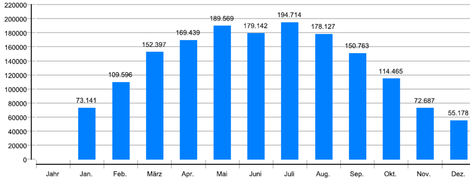
Ertrag Photovoltaik AC [Qinv]
