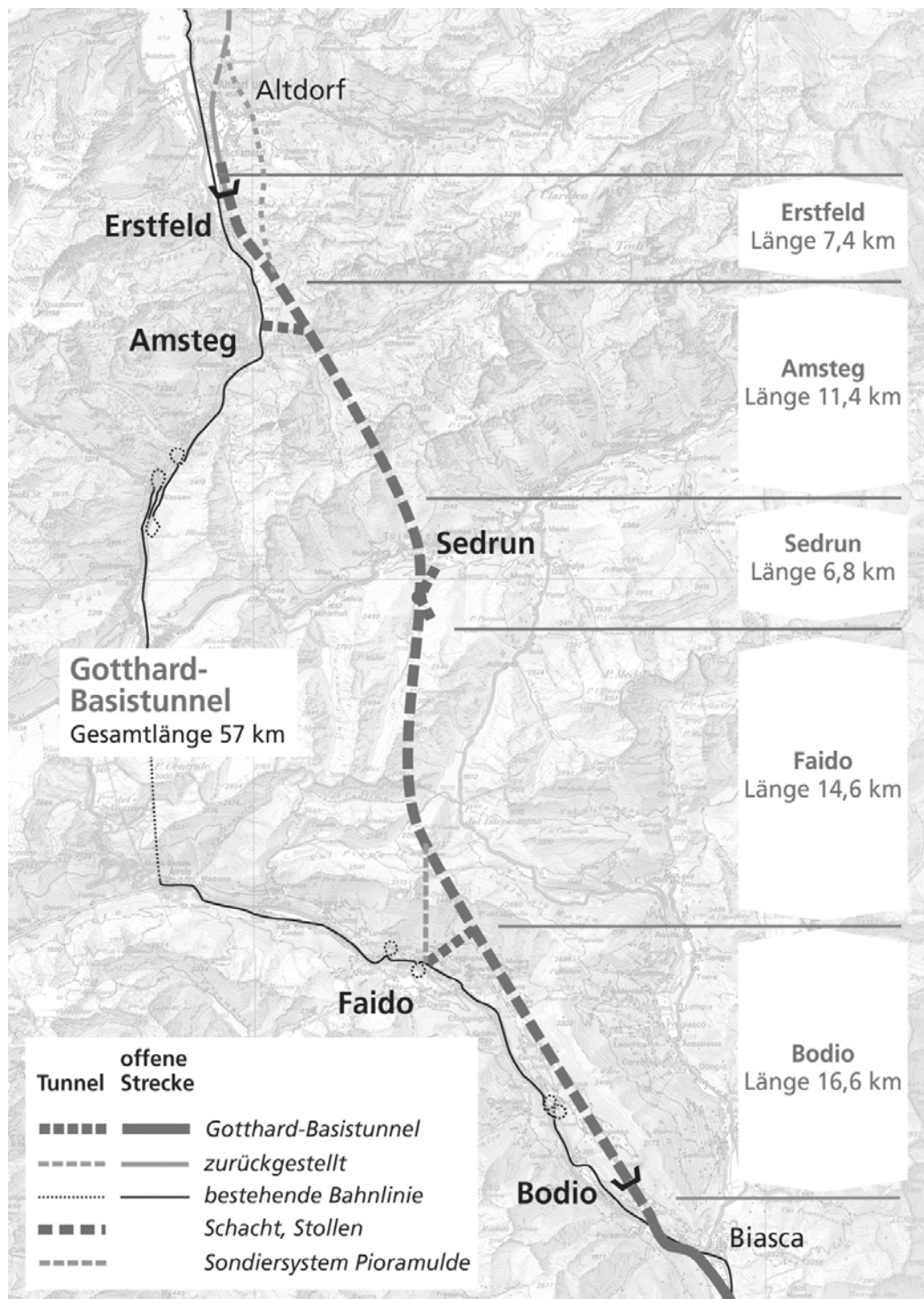
Abb. 1: Gotthard-Basistunnel, Situationsplan
