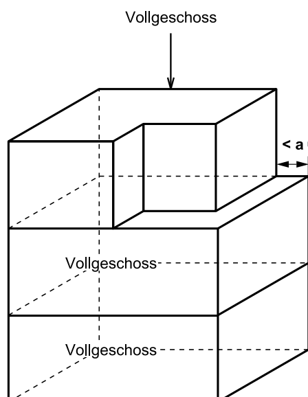
Figur 6.4 Attikageschosse
